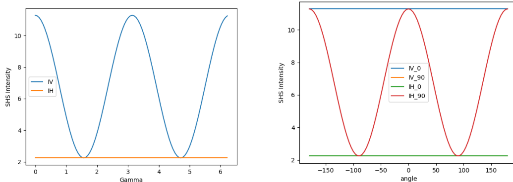
Figure 4: Polarization resolved HRS (left) and angle resolved HRS (right)
